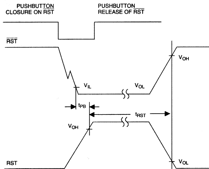
PUSHBUTTON RESET TIMING Figure 4
