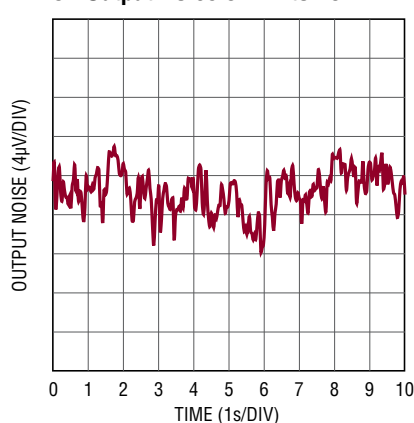
5V Output Noise 0.1Hz to 10Hz
