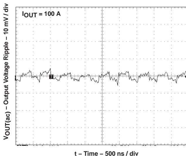
Figure 11. Output Noise
