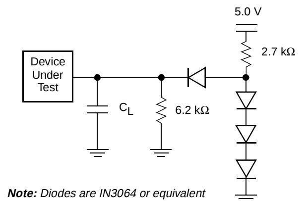
Figure 6. Test Setup
