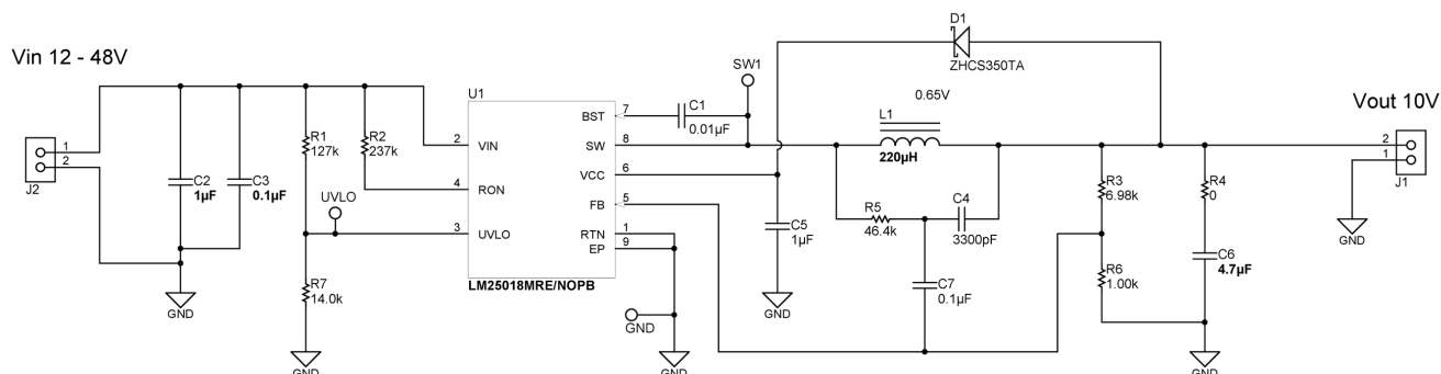
Figure 1. Complete Evaluation Board Schematic for LM25018 Based Synchronous Buck Converter
