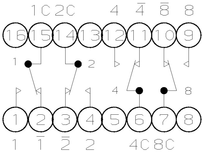
SCHEMATIC (POSITION 0)
