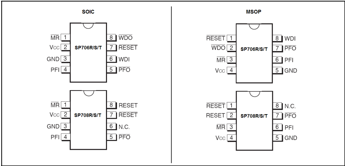
Fig. 3: Pin Assignment
