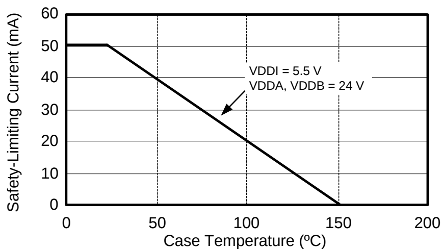
Figure 7. WB SOIC-16, NB SOIC-16, 14 LD LGA Thermal Derating Curve, Dependence of Safety Limiting Values with Case Temperature per DIN EN 60747-5-5
