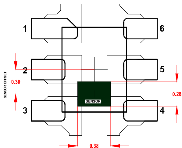
FIGURE 17. 6 LD ODFN SENSOR LOCATION OUTLINE
