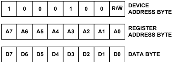
FIGURE 10. DEVICE ADDRESS, REGISTER ADDRESS AND DATA BYTE
