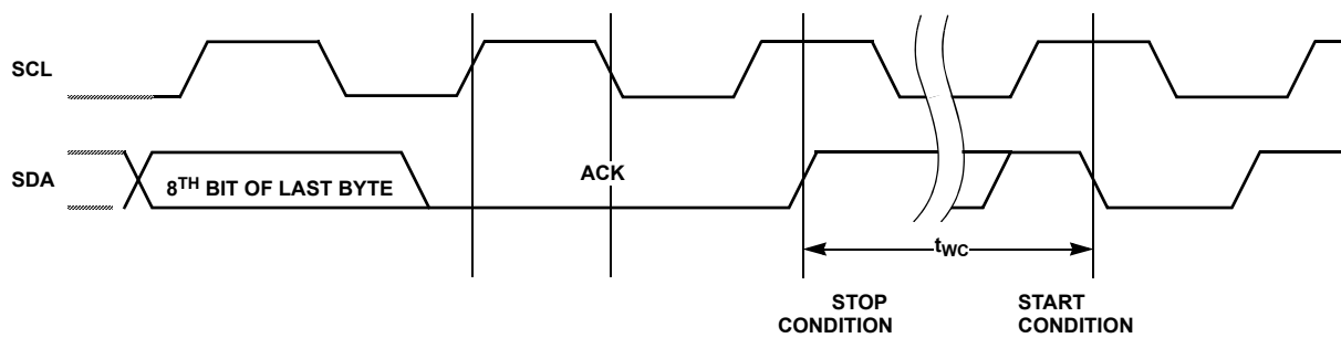
FIGURE 5. I 2 C WRITE CYCLE TIMING
