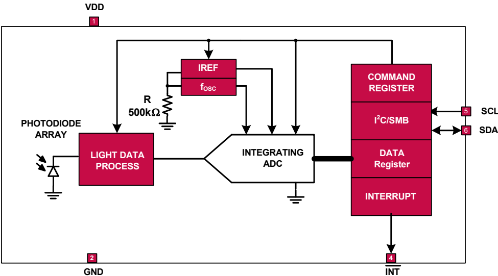
FIGURE 3. BLOCK DIAGRAM
