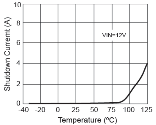
Figure 2. Shutdown Current vs. Temperature
