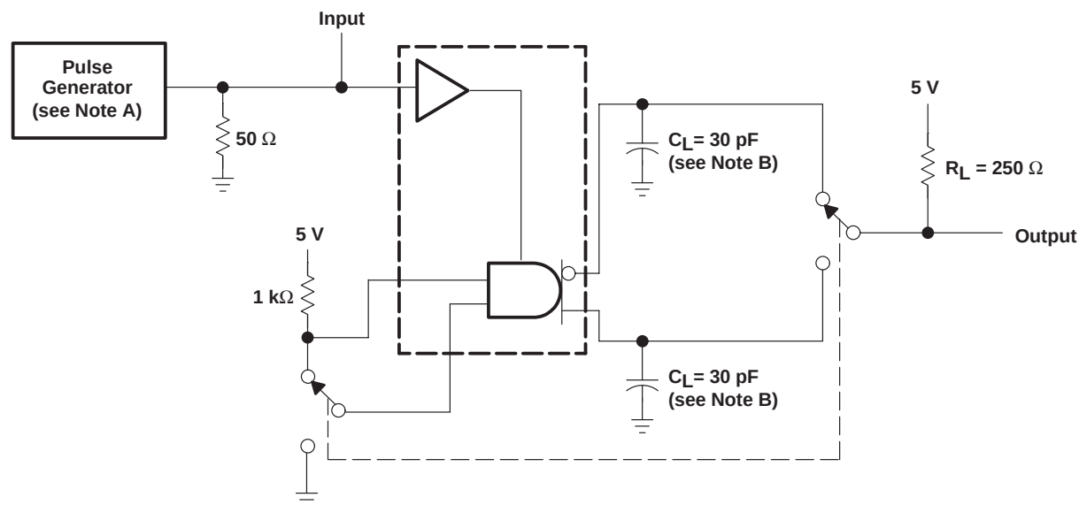
TEST CIRCUIT
