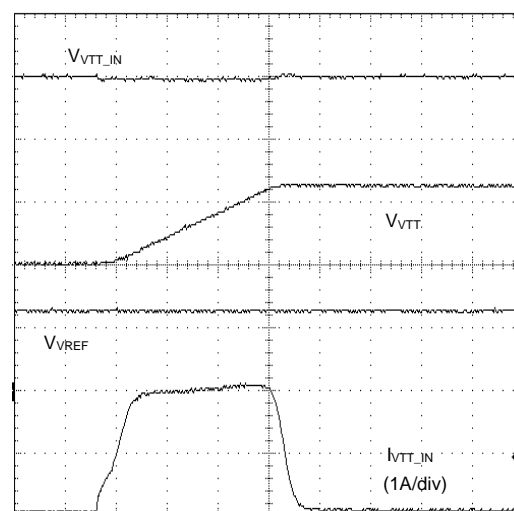
Figure 8. Start-up Waveform
