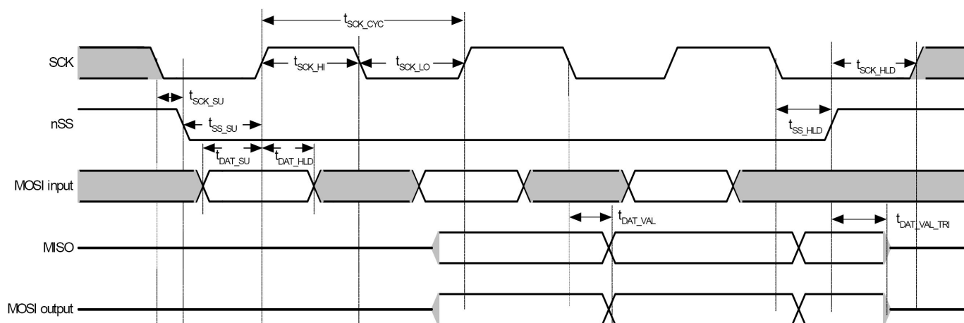
Figure 7 - SPI Timing
