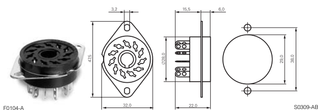
MT 78 613 Socket 11-pin with solder terminals
