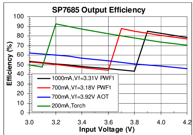
Figure 2. Output Efficiency
