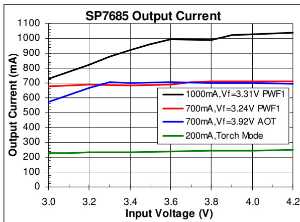
Figure 1. Output Current
