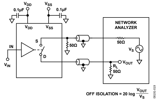
Figure 19. Off Isolation
