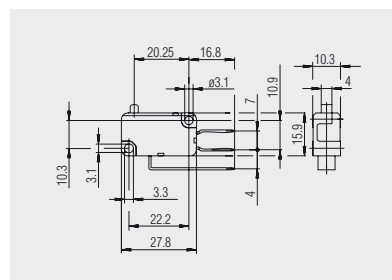
Quick-connect terminal 6.3 PITCH 7
