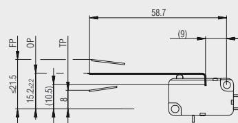
L03: straight lever
