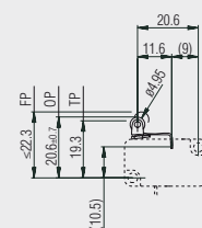
L11: roller lever 191.079.013
