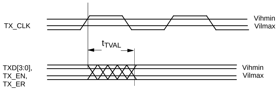
Figure 80. Transmit Timing
