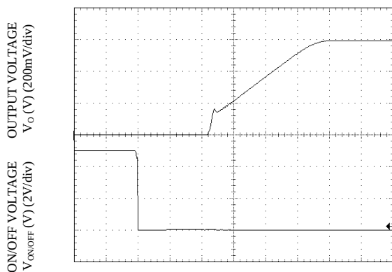
Start-up Using On/Off Voltage ( I_o = I_{o,max} ), V_o=0.8V
