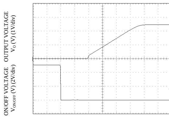
Start-up Using On/Off Voltage ( I_o = I_{o,max} ), V_o=2.5V
