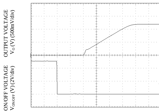
Start-up Using On/Off Voltage ( I_o = I_{o,max} ), V_o=1.2V
