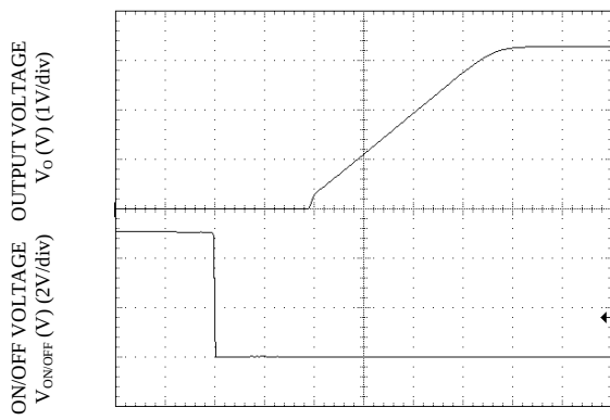
Start-up Using On/Off Voltage ( I_o = I_{o,max} ), V_o=3.3V
