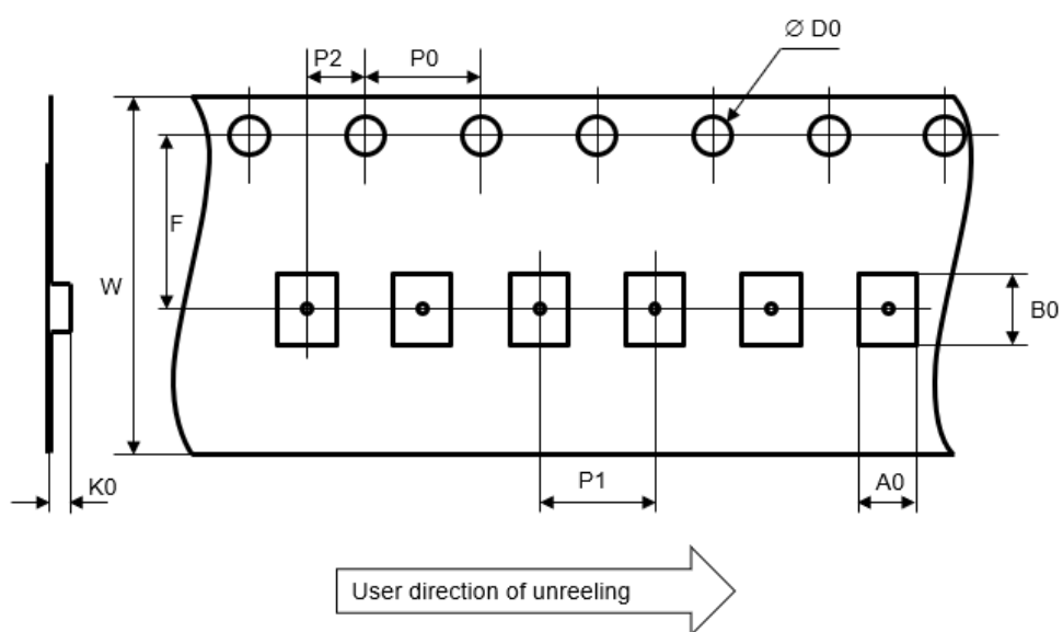
Figure 12. Tape outline
