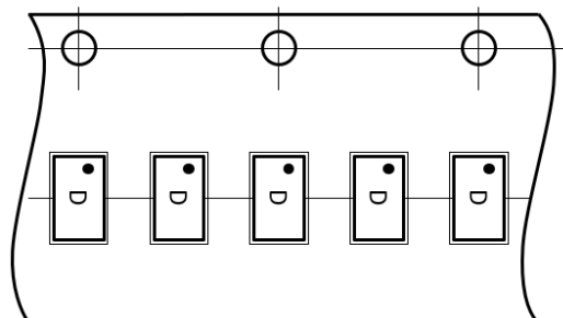
Figure 11. Package orientation in reel
