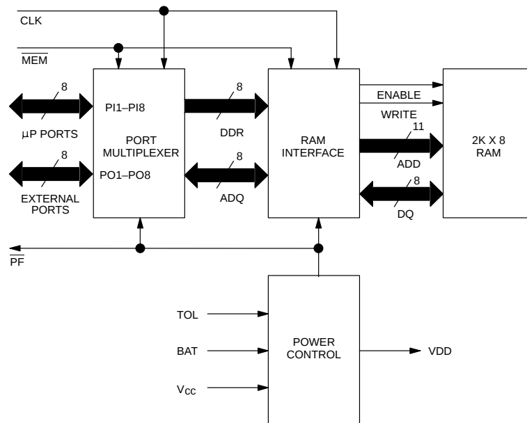
FUNCTIONAL BLOCK DIAGRAM Figure 1
