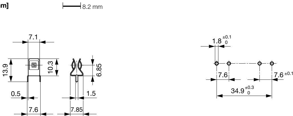
Drilling diagram
