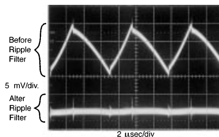
FIGURE 17. Post Ripple Filter Waveform
