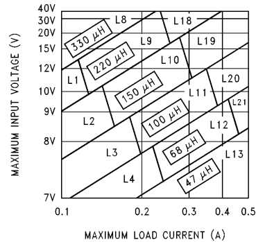
FIGURE 6. LM2594-5.0
