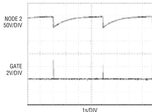
Figure 10. Automatic Restart After Current Fault
