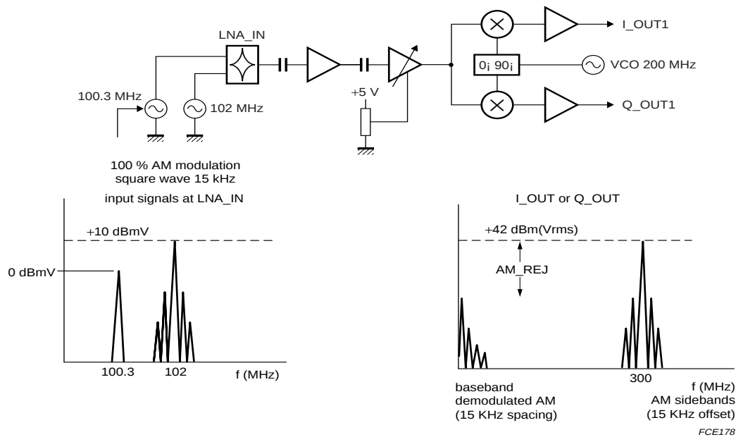
Fig.9 Overall AM rejection measurement.
