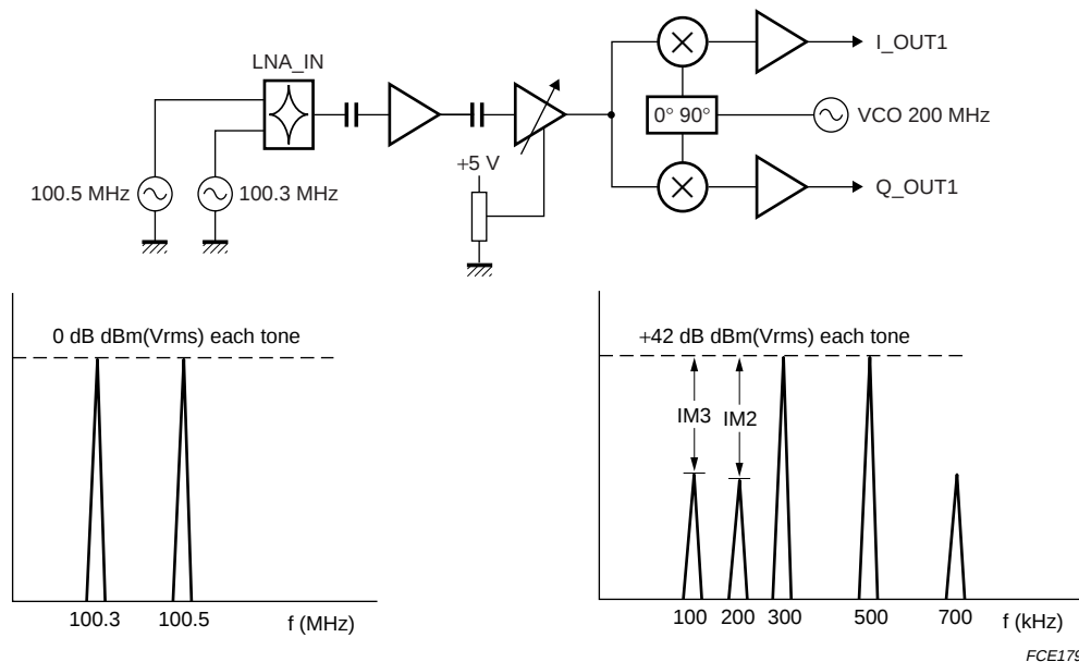
Fig.10 Overall IM3 measurement.
