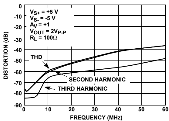
FIGURE 8. DISTORTION vs FREQUENCY ( A_V = +1 )
