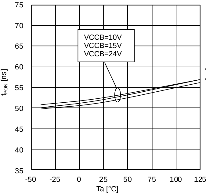
Figure 44. Turn ON Time (INA=L, INB=PWM, BM60210FV)
