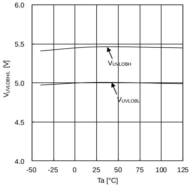
Figure 57. VCCB UVLO ON/OFF voltage (BM60211FV)
