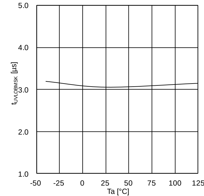
Figure 58. VCCB UVLO mask time (BM60210FV)
