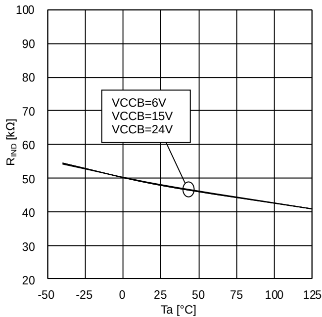
Figure 25. logic pull-down resistance (BM60211FV)
