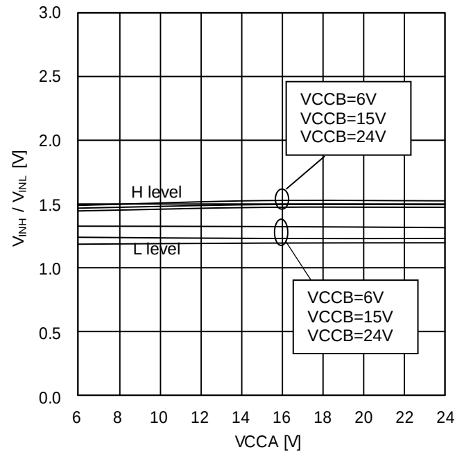
Figure 21. logic(INA/INB)H/L level input voltage (BM60211FV)
