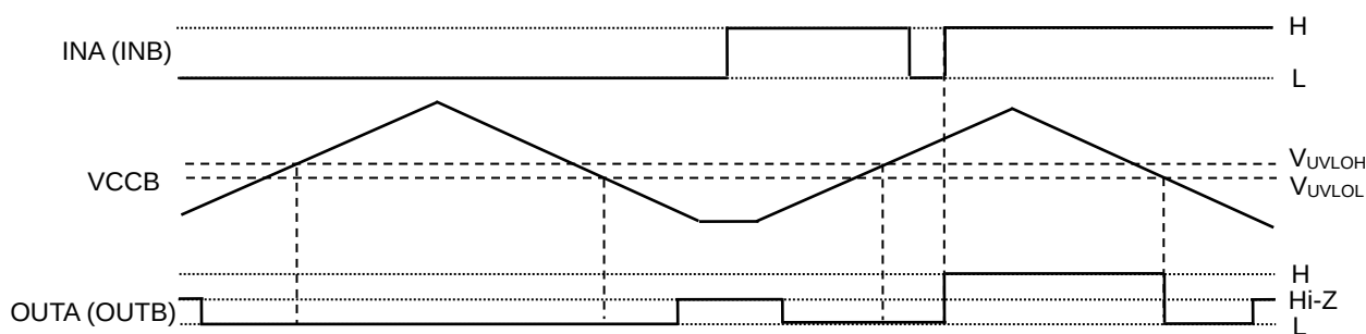
Figure 5. Output-side UVLO Function Operation Timing Char
