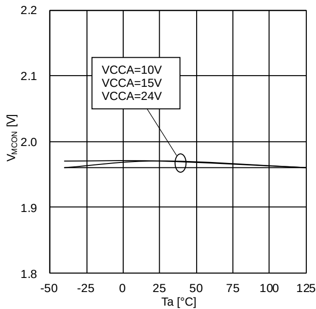
Figure 52. MCA ON threshold (BM60210FV)
