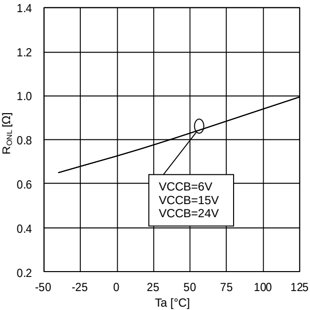
Figure 39. OUTB ON resistance (Sink, BM60211FV)
