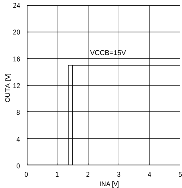
Figure 23. OUT_A output voltage vs INA input voltage ( V_{CCB}=15V , V_{CCA}=15V , T_a=25^{\circ}C , BM60211FV)
