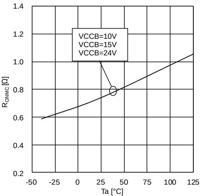
Figure 50. MCB ON resistance (BM60210FV)
