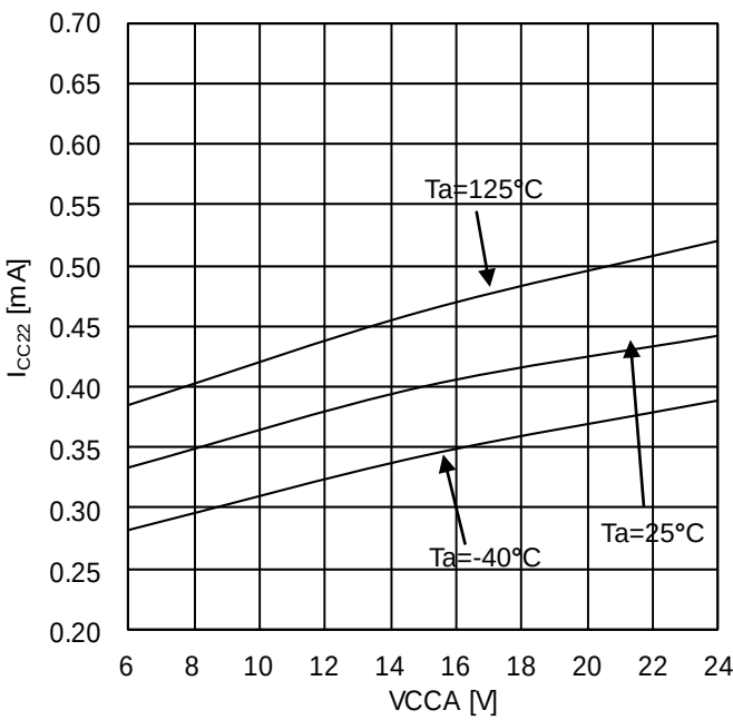
Figure 19. VCCA circuit current 2 (OUTA=H, BM60211FV)
