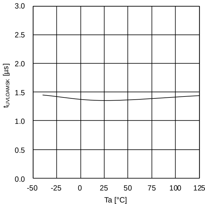
Figure 63. VCCA UVLO mask time (BM60211FV)
