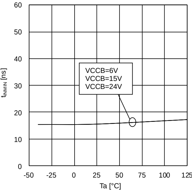
Figure 29. log(INA)input mask time (BM60211FV)
