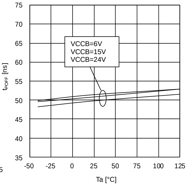
Figure 47. Turn OFF Time (INA=L, INB=PWM, BM60211FV)
