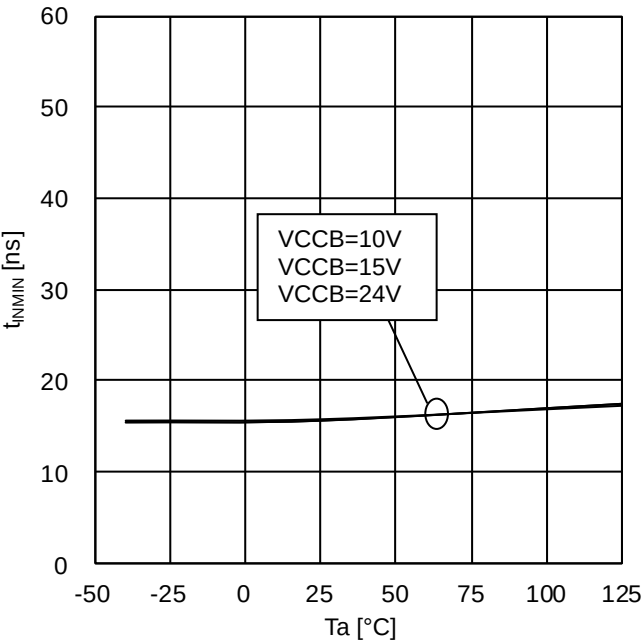
Figure 28. log(INA)input mask time (BM60210FV)
