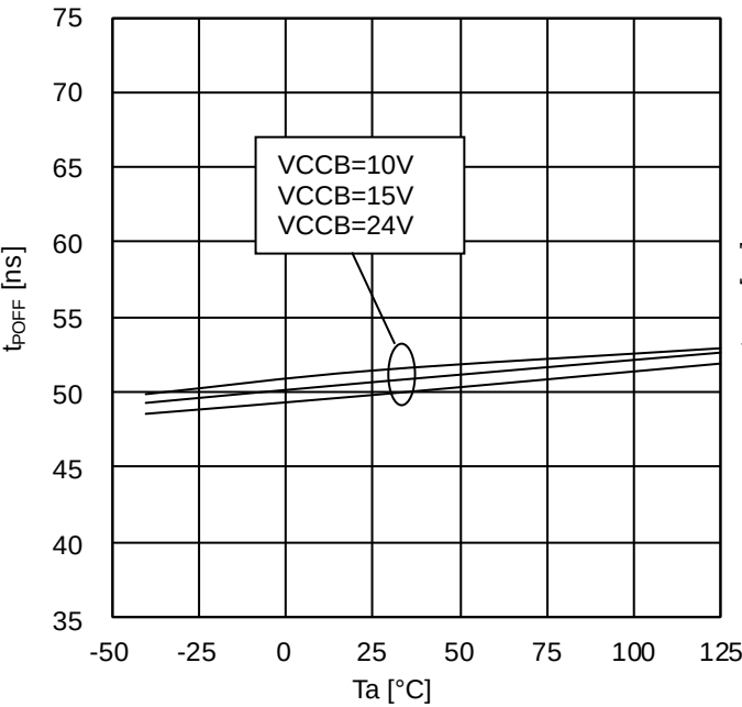
Figure 46. Turn OFF Time (INA=L, INB=PWM, BM60210FV)
