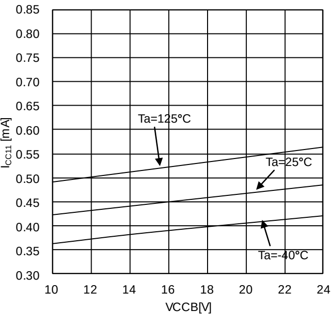
Figure 8. VCCB circuit current 1 (OUTB=L, BM60210FV)
