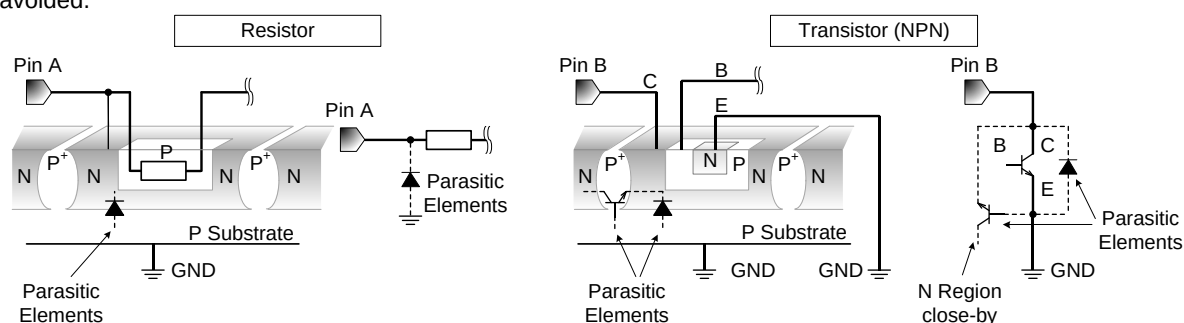
Figure 64. Example of IC structure
