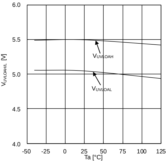
Figure 61. VCCA UVLO ON/OFF voltage (BM60211FV)
