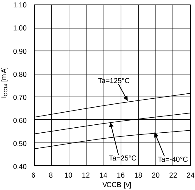
Figure 15. VCCB circuit current 4 (INA=20kHz, Duty=50%, BM60211FV)
