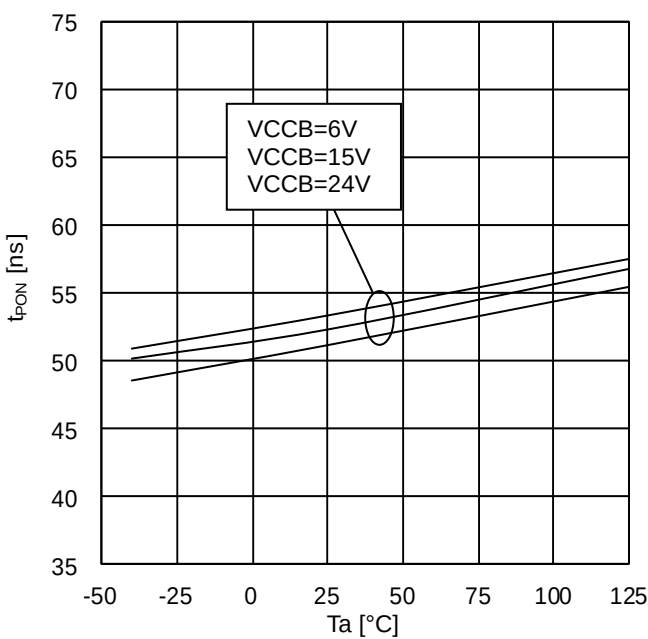
Figure 41. Turn ON Time (INA=PWM, INB=L, BM60211FV)
