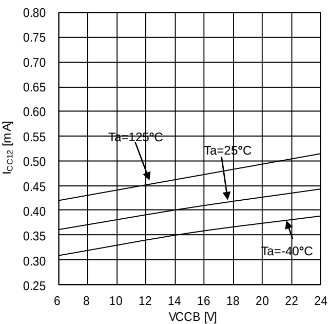
Figure 11. VCCB circuit current 2 (OUTB=H, BM60211FV)
