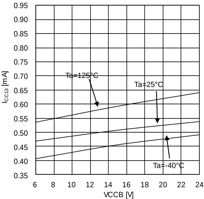
Figure 13. VCCB circuit current 3 (INA=10kHz, Duty=50%, BM60211FV)
