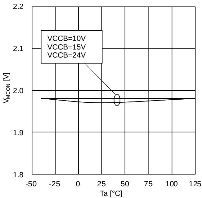
Figure 54. MCB ON threshold (BM60210FV)
