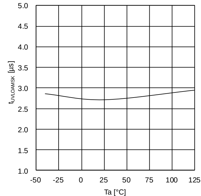
Figure 62. VCCA UVLO mask time (BM60210FV)
