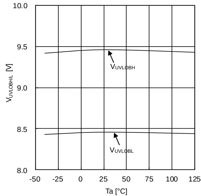
Figure 56. VCCB UVLO ON/OFF voltage (BM60210FV)
