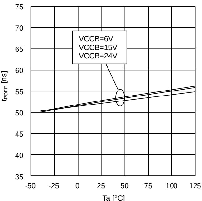
Figure 43. Turn OFF Time (INA=PWM, INB=L, BM60211FV)
