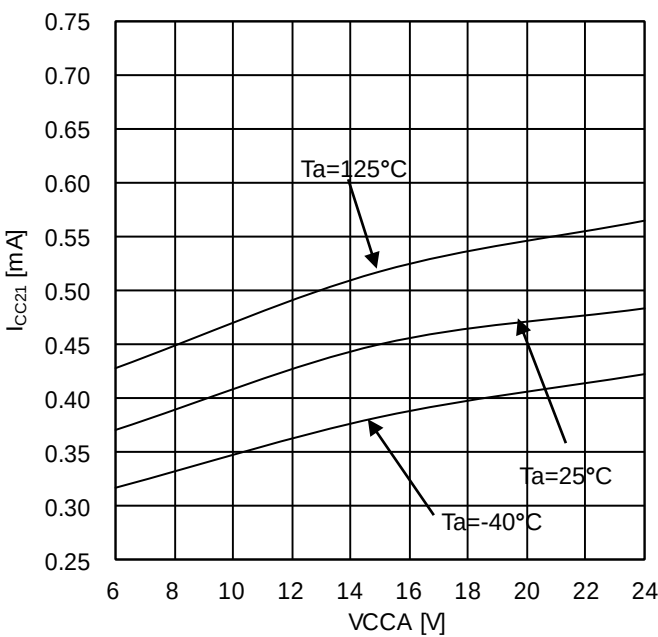
Figure 17. VCCA circuit current 1 (OUTA=L, BM60211FV)
