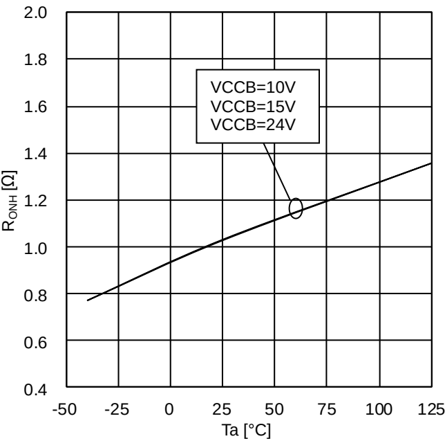
Figure 36. OUTB ON resistance (Source, BM60210FV)
