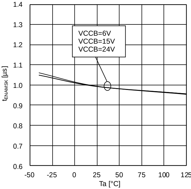
Figure 31. ENA input mask time (BM60211FV)
