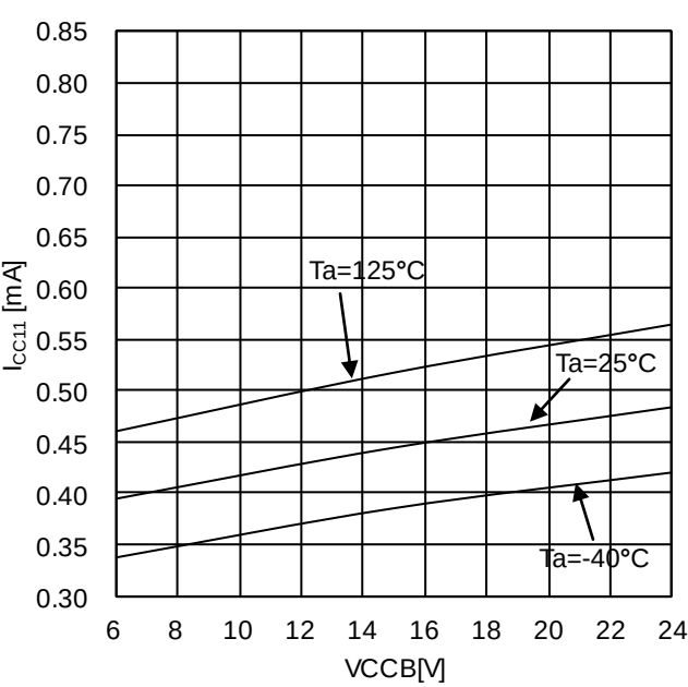
Figure 9. VCCB circuit current 1 (OUTB=L, BM60211FV)
