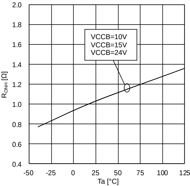
Figure 37. OUTB ON resistance (Source, BM60211FV)
