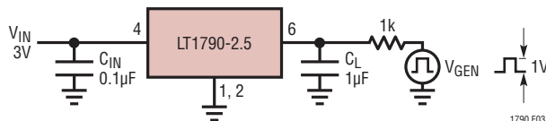
Figure 3. Response Time Test Circuit
