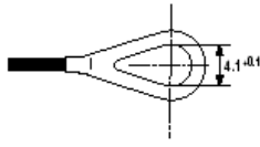
Square flange receptacle cap end
