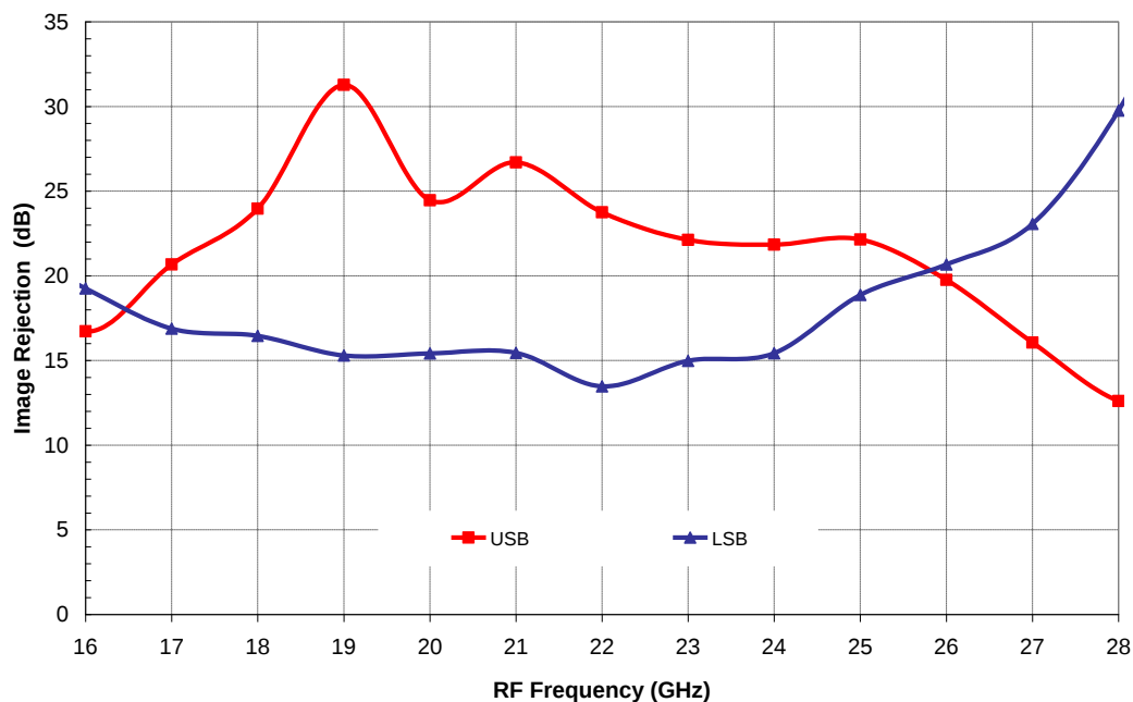
Image Rejection on Supradyne & Infradyne Mode versus Frequency
