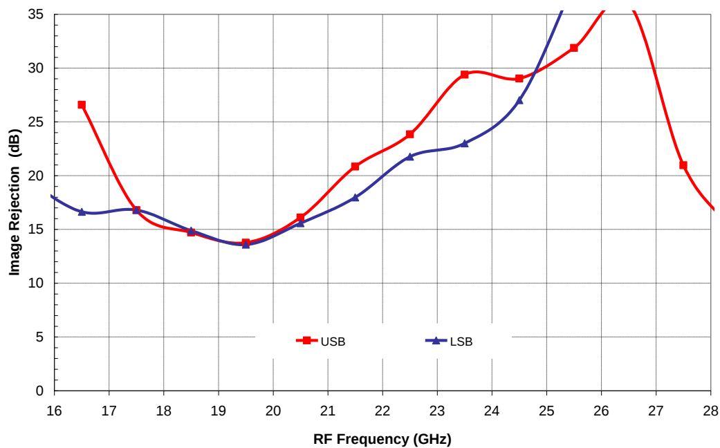
Image Rejection on Supradyne & Infradyne Mode versus Frequency
