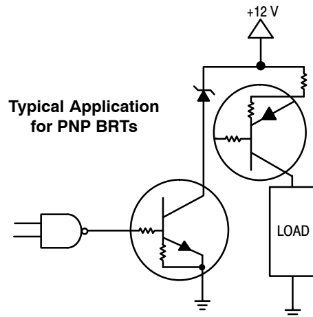
Figure 42. Inexpensive, Unregulated Current Source
