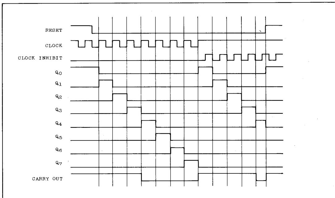
TIMING CHART
