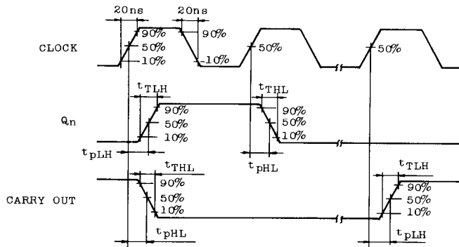
WAVEFORM 1.
