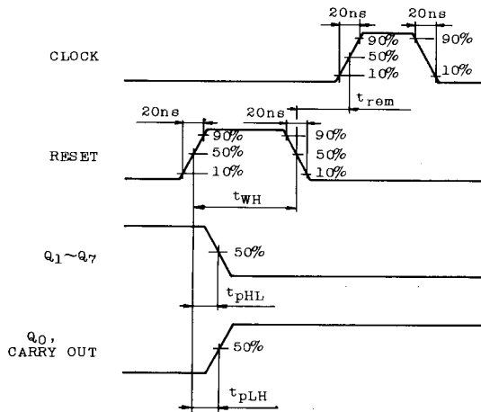
WAVEFORM 2.
