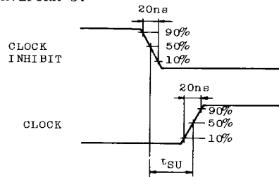
WAVEFORM 3.
