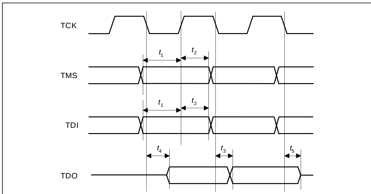
Figure 47 JTAG Timing
