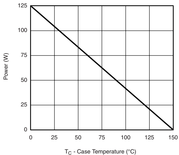
Power, Junction-to-Case
