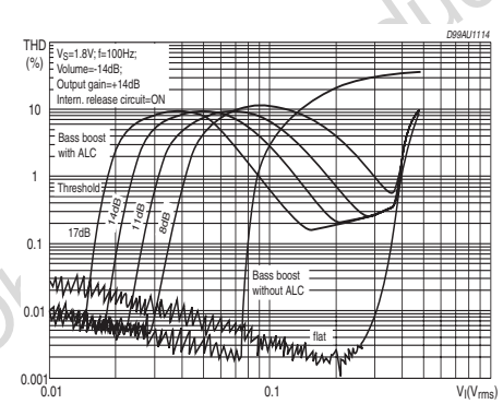
Figure 13. BASS ALC: THD
