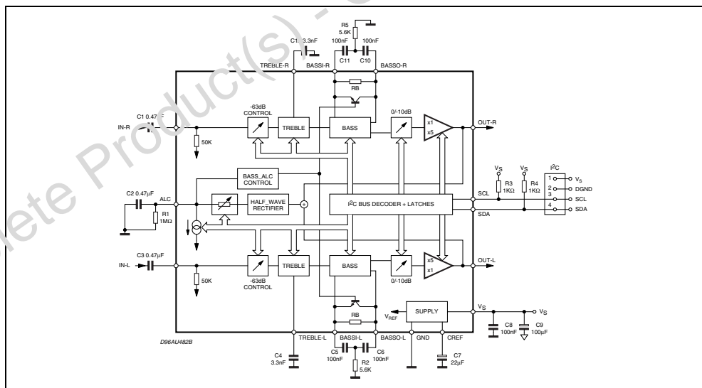
Figure 2. Block Diagram
