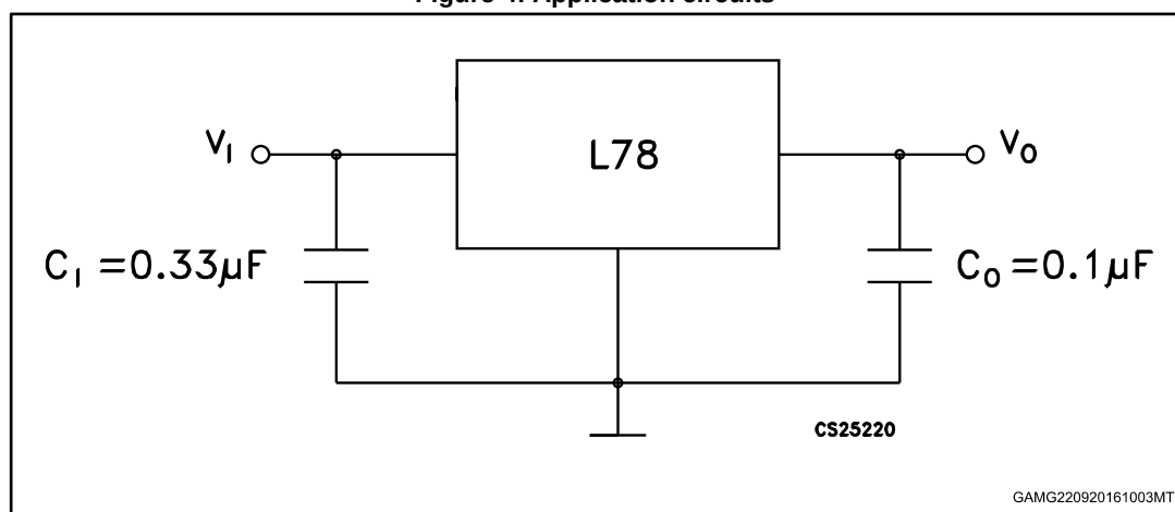
Figure 4: Application circuits
