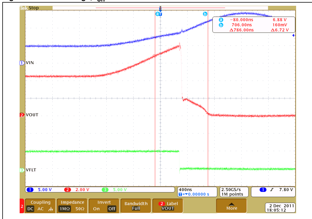
Figure 11. Overvoltage, t_{off}
