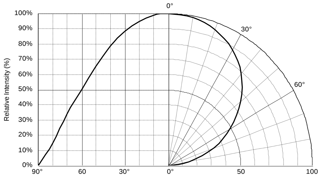
Fig 4. Radiation Characteristics
