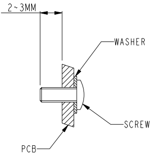
DETAIL 2 RECOMMENDED SCREW LENGTH
