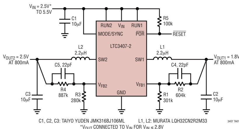
Figure 1. 2.5V/1.8V at 800mA Step-Down Regulators
