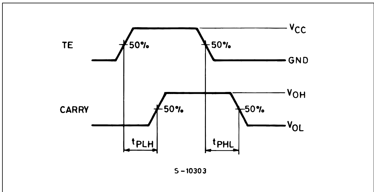
WAVEFORM 5 : PROPAGATION DELAY TIME ( f=1\text{MHz} ; 50% duty cycle)
