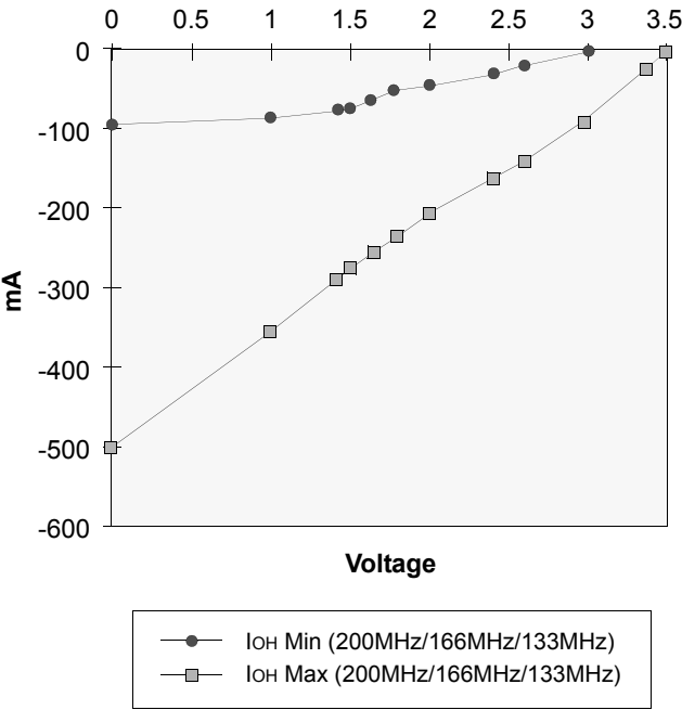
Figure 4. 200MHz/166MHz/133MHz Pull-up
