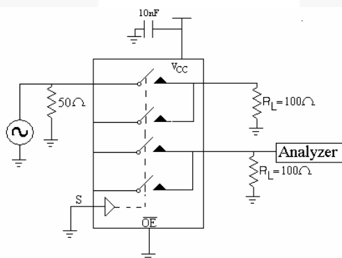
Figure 8. Crosstalk
