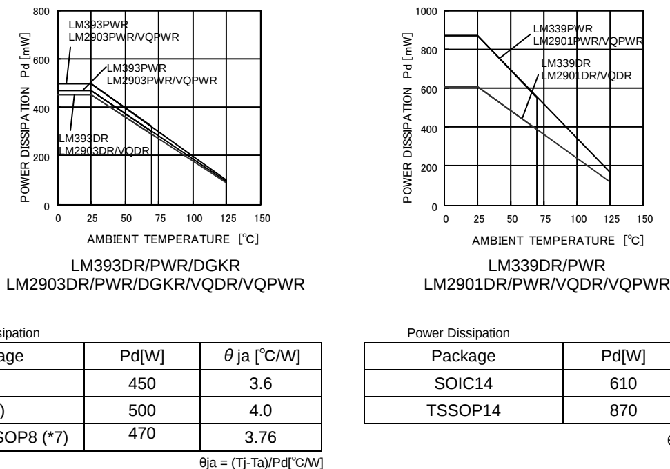
Fig.91 Derating Curves
