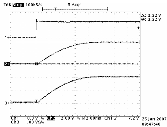
Figure 13- Start up 2A, ch1: VIN; ch2: VOUT; ch3: IOUT
