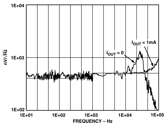
TPC 6. Noise Spectral Density
