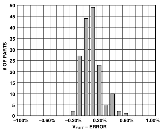
TPC 2. Typical Output Voltage Error Distribution
