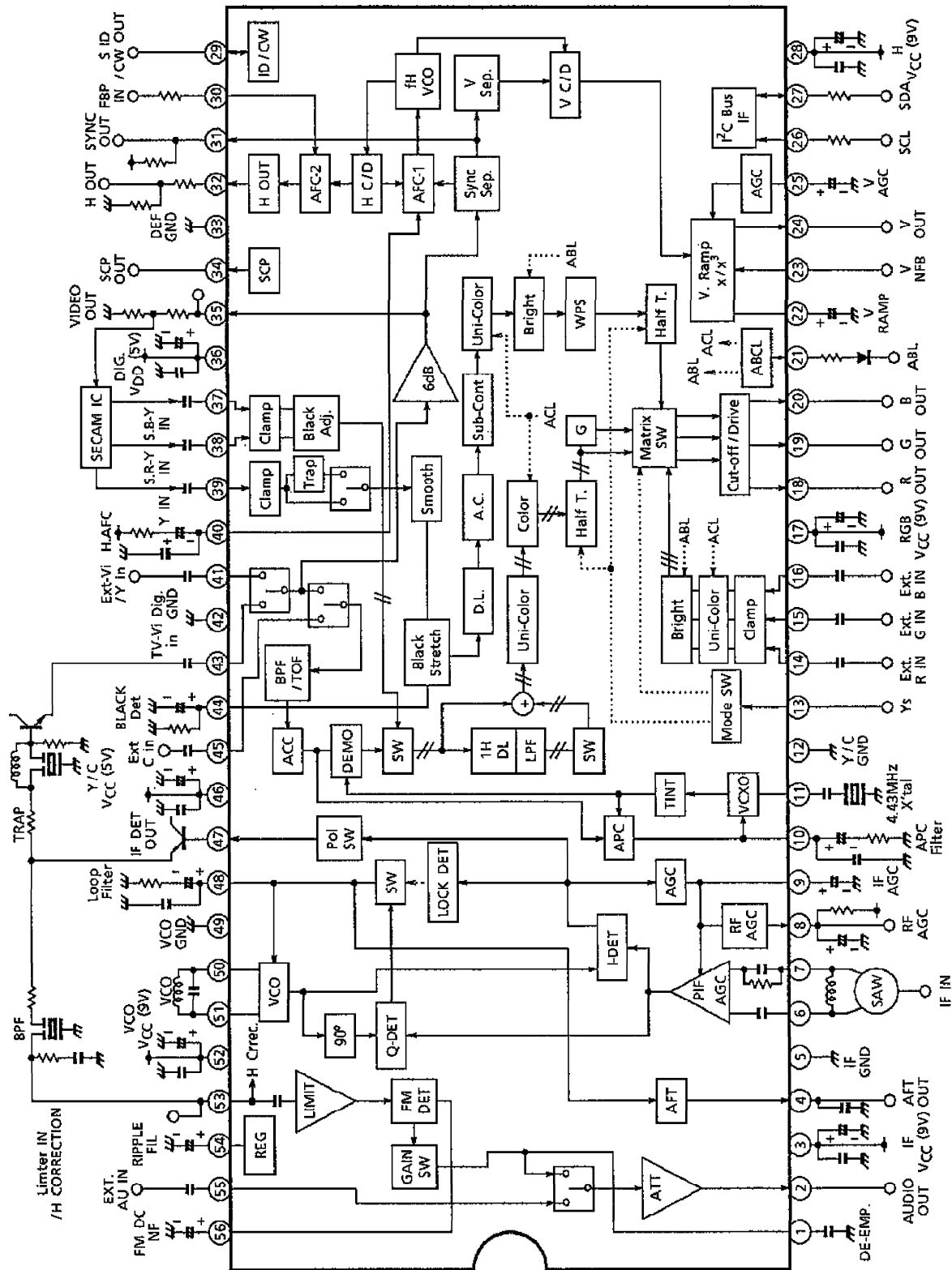
BLOCK DIAGRAM
