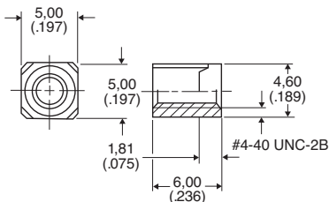
Rectangular Nut
