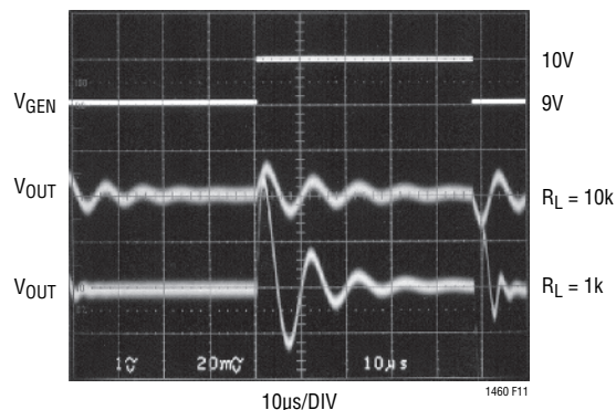
Figure 11. C_L = 0.01\mu\text{F}
