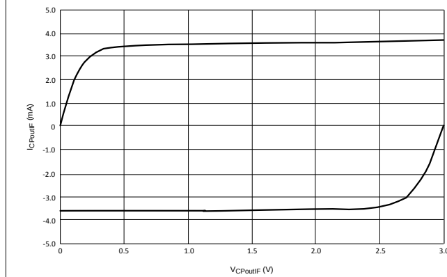
Figure 15. IF PLL Charge Pump Current
