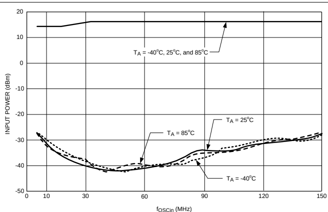
Figure 7. OSCin Sensitivity
